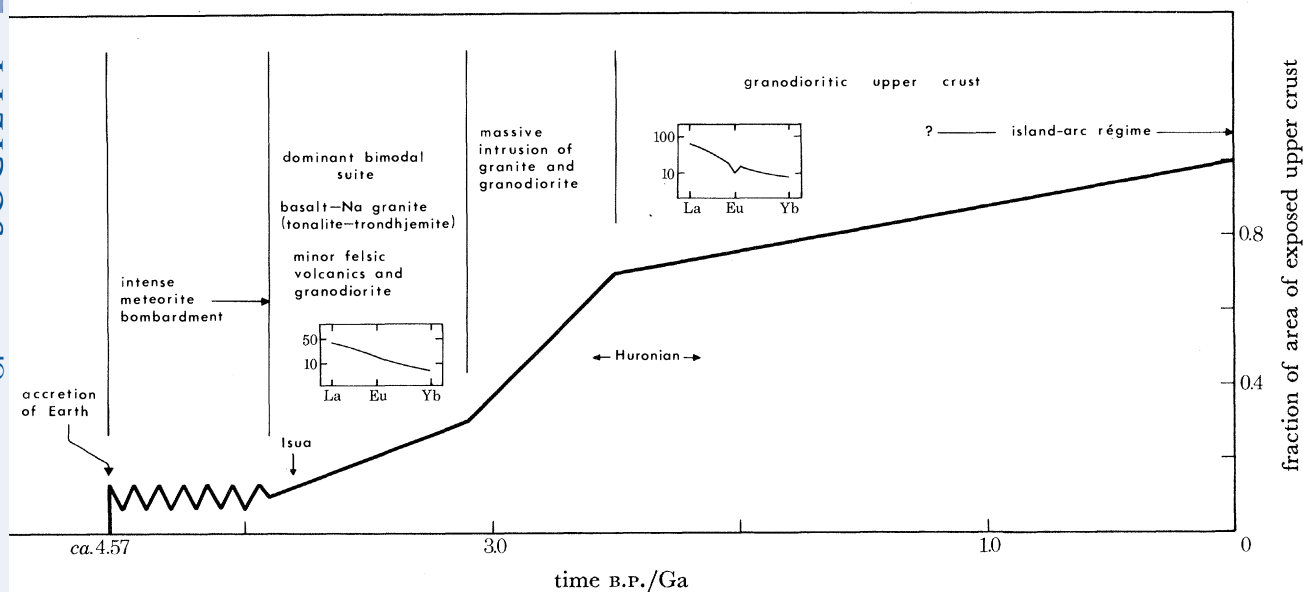
FIGURE 7. Model for the evolution of the continental crust throughout geological time. Average sedimentary r.e.c. patterns are indicated, as are some of the principal events of crustal evolution. The changes in upper-crustal composition, and a massive increase in continental growth, takes place between 3.0 and 2.5 Ga B.P. This change will be reflected a little later in the sedimentary record (e.g. Huronian, cf. figure 6).
