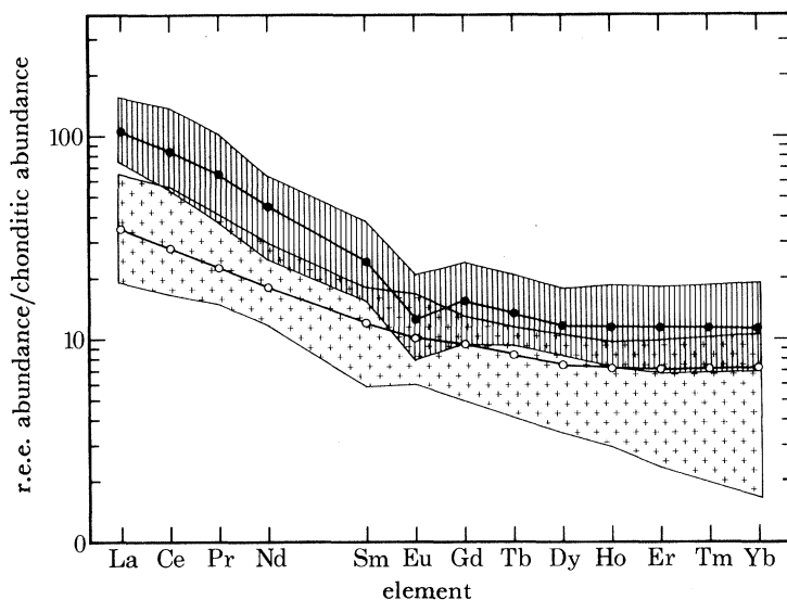
FIGURE 2. R.e.e. patterns, normalized to chondritic abundances (C-1, volatile-free), for the post-Archaean average Australian sedimentary rocks (p.A.a.s., ●), and for the average Archaean sedimentary rocks a.A.s., ○). The fields for individual samples of typical Archaean (a.A.s., +) and post-Archaean (p.A.a.s., ||||) sedimentary rocks are also shown. Data from Nance & Taylor (1976, 1977), Bavington & Taylor (1980), from this laboratory. (Reproduced from Taylor & McLennan (1980a).)
