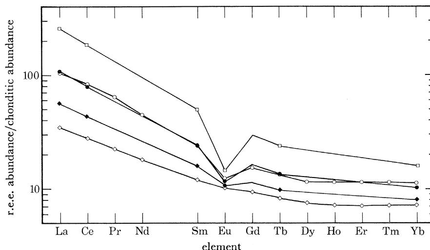
FIGURE 3. R.e.e. patterns, normalized to chondritic abundances (C-1, volatile-free) for p.A.a.s., a.A.s. and 36 late Archaean K-rich granites (Taylor & McLennan 1981 a ); \circ , p.A.a.s.; \diamond , a.A.s.; \square , K granite; \bullet , 2 a.A.s.: 1 K granite mixture; \blacklozenge , 9 a.A.s.:1 K granite mixture. Note that even 10% of K-rich granite patterns mixed with a.A.s. produces a discernible Eu depletion. This indicates that K-rich granites are not a significant source for average Archaean sedimentary rocks. A mix of two-thirds a.A.s. and one-third granite produces r.e.e. patterns similar to p.A.a.s. (Reproduced from Taylor & McLennan (1981 a ).
